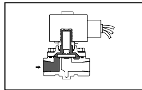
Figure 3A: Pilot Operated, Normally Closed Valve, De-Energized
